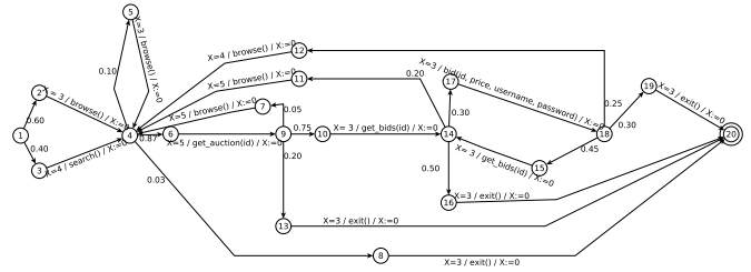
Figure 1: Example of a probabilistic timed automata
