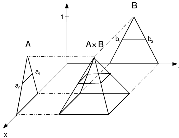
Figure 1: Non-interactive possibility distributions.
