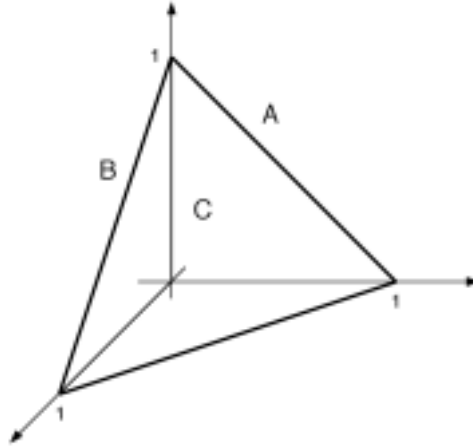
Figure 5: The case of \rho_f(A, B) = 1/3 .
