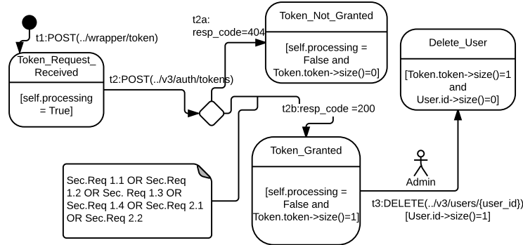
Fig. 4. Behavioral Model for KS Security Wrapper(SecKS)
