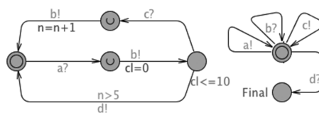
Figure 1: Example of an UTA model
