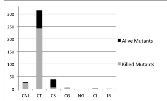
Figure 5: The proportion of alive and killed mutants for each mutation operator
