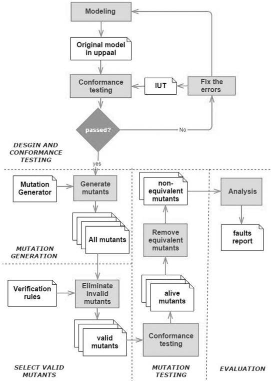
Figure 2: Our approach of Specification Mutation Testing
