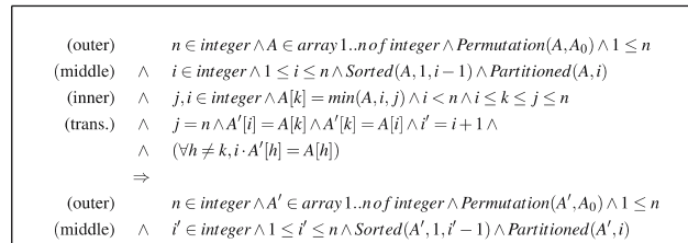
Fig. 16. Verification condition
