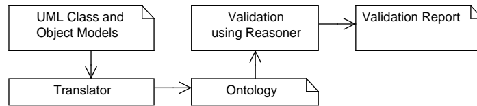
Fig. 2. Automatic object and class model conformance process.
